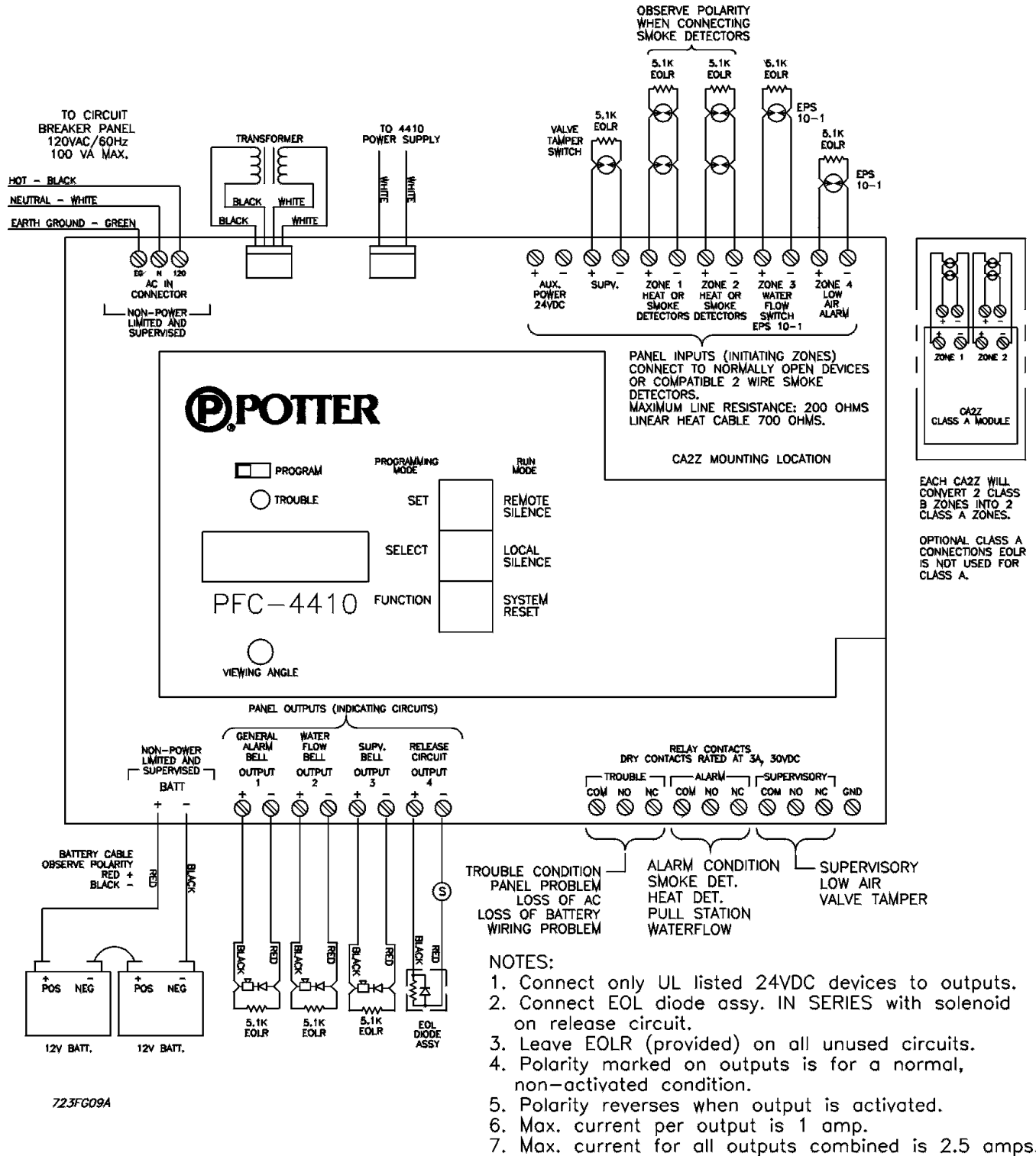
Figure 9 - Wiring Diagram
