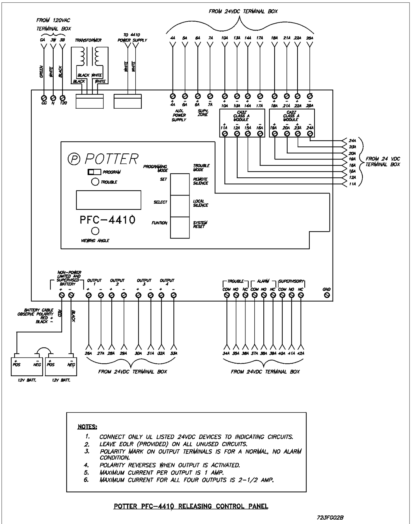
Figure 2 — Wiring Diagram 5.
