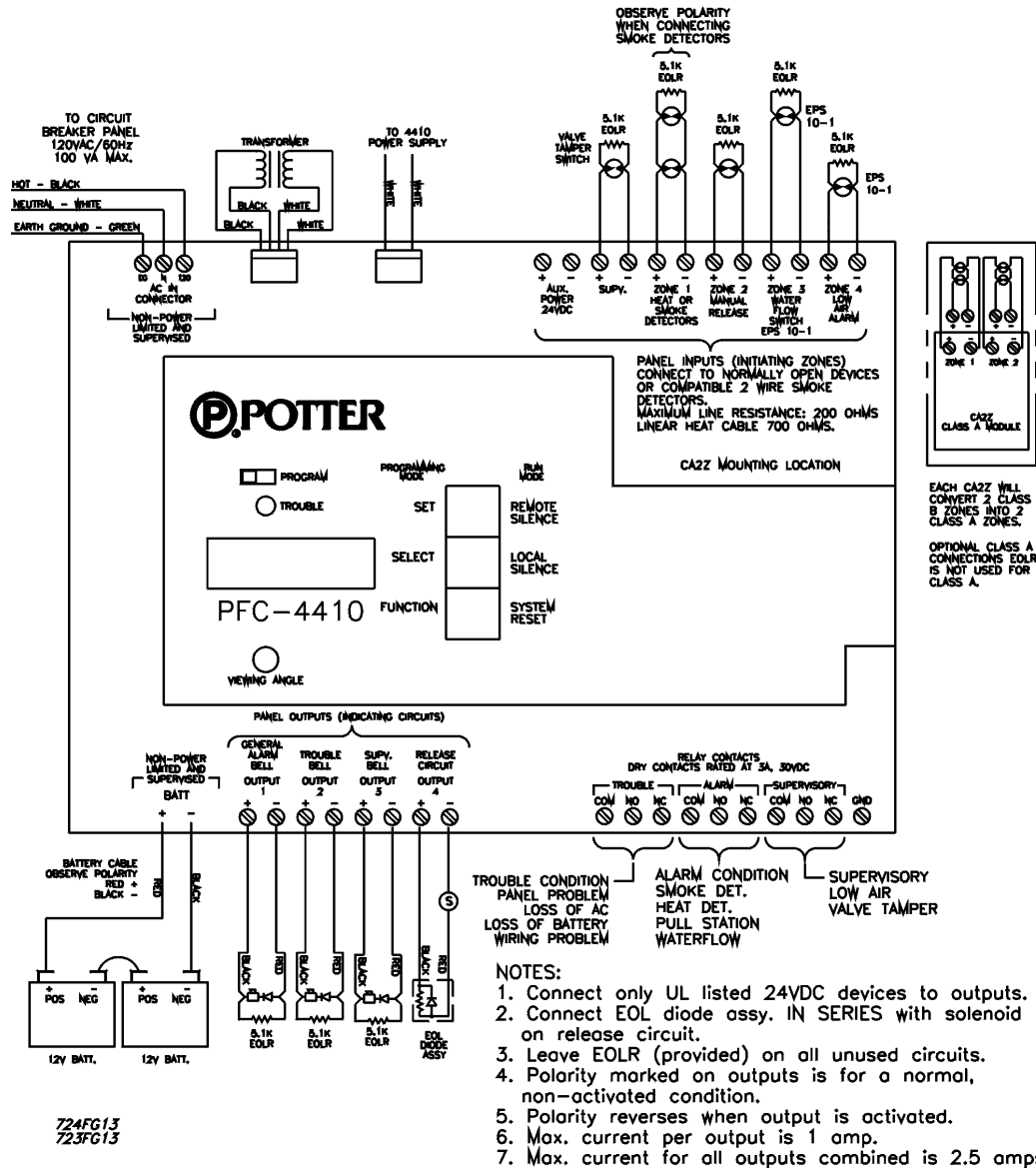
Figure 13 — Wiring Diagram
