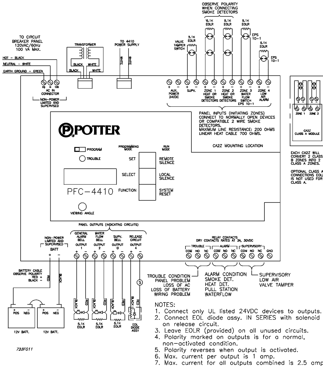
Figure 11 — Wiring Diagram
