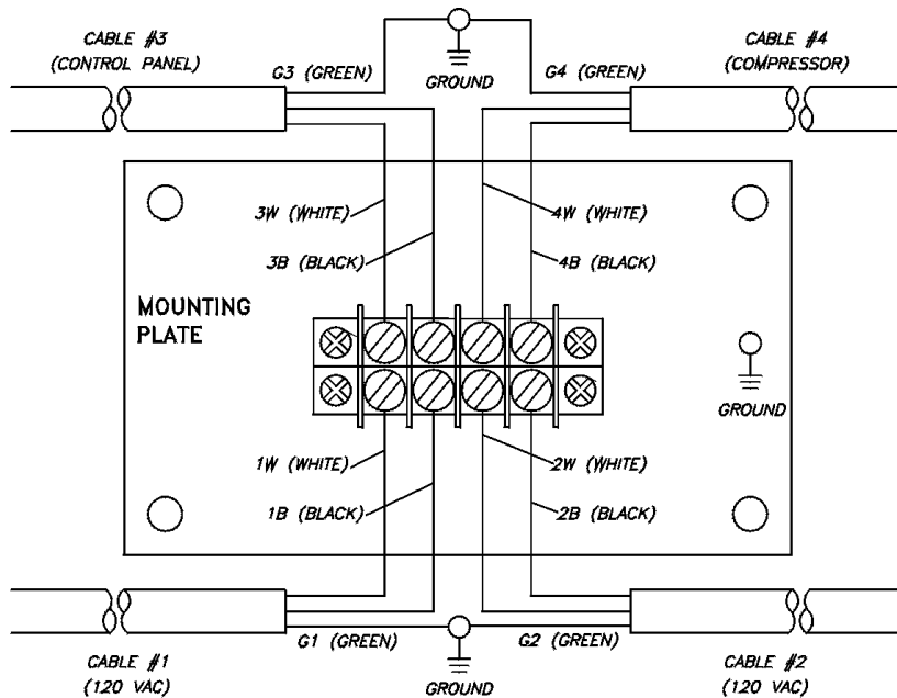
120 VAC TERMINAL BOX (FACTORY CONNECTIONS)
