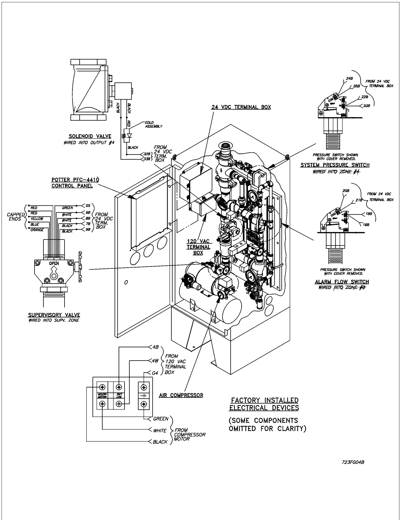
Figure 4 — Wiring Diagram
