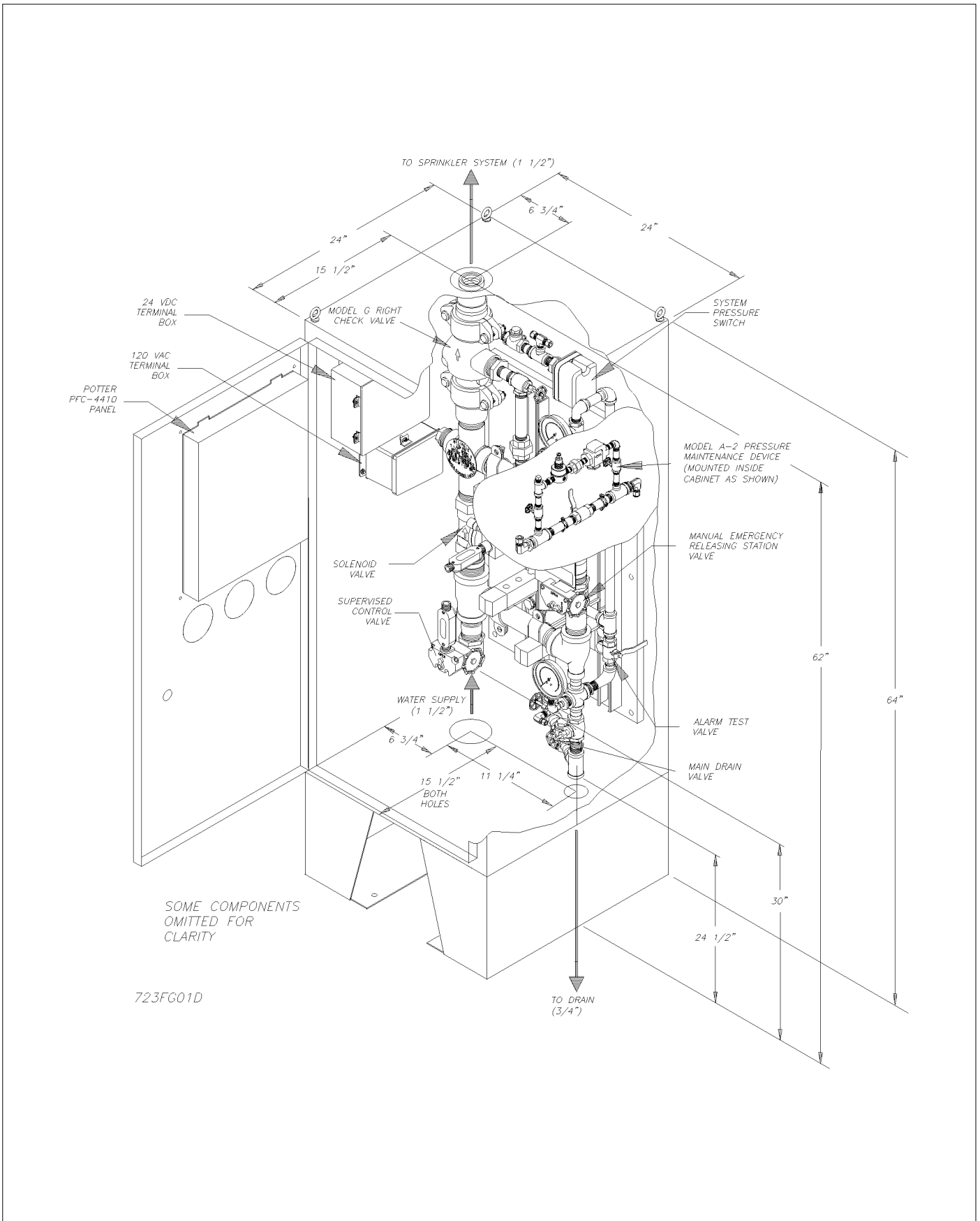
Figure 1 — Installation Dimensions
