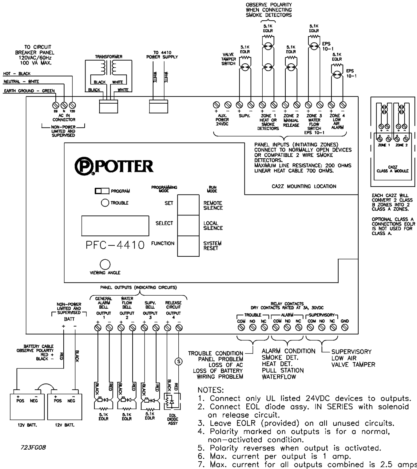
Figure 8 - Wiring Diagram
